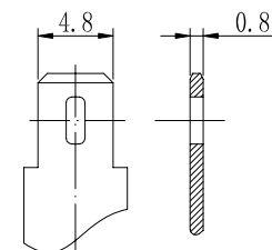
Terminal T1
