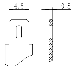
Terminal T1
