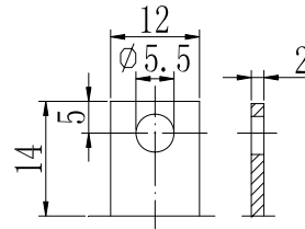
Terminal T3
